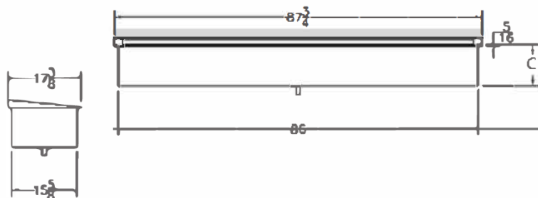
SIDE ELEVATION
