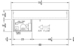
FRONT VIEW (OPERATOR SIDE)
