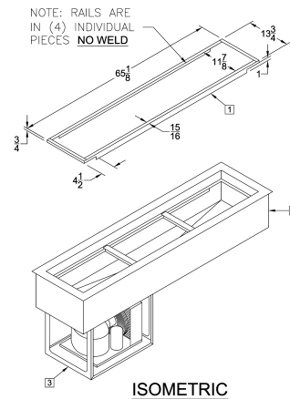
ISOMETRIC
